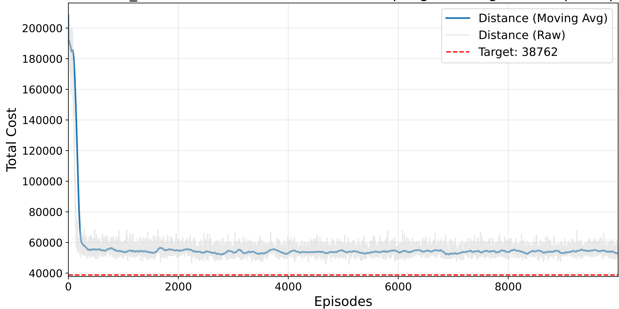
Final NO_MASK Masked AutoRL-SOP (Resampling) Training - kro124p.1.sop
